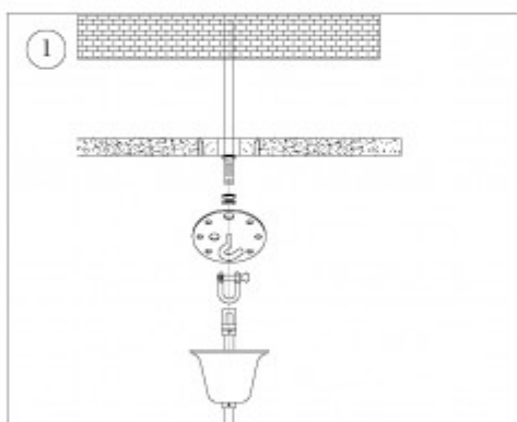
Hang the ceiling tray on the ceiling
