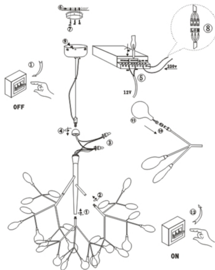
EVITA SP36 GOLD TRANSPARENT
